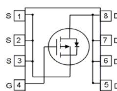
PG-DSO-8
